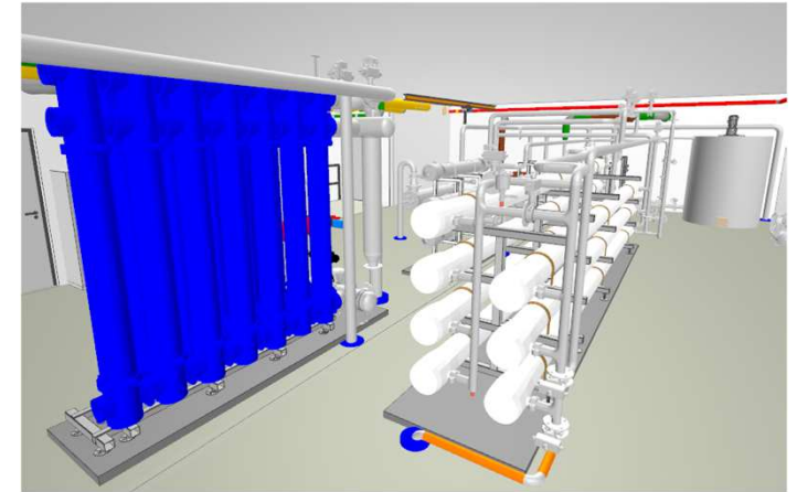
Membranfiltration
